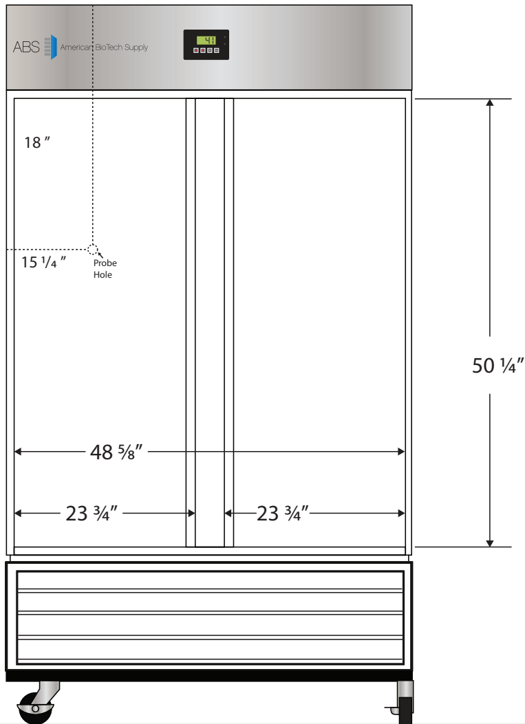
Front View
