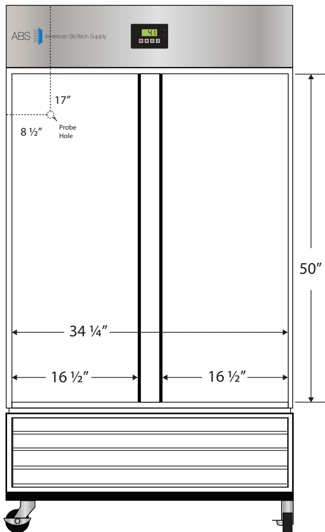
Front View
