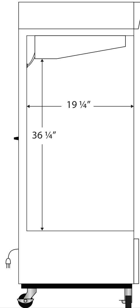
Side View
