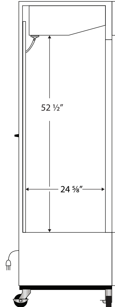
Side View
