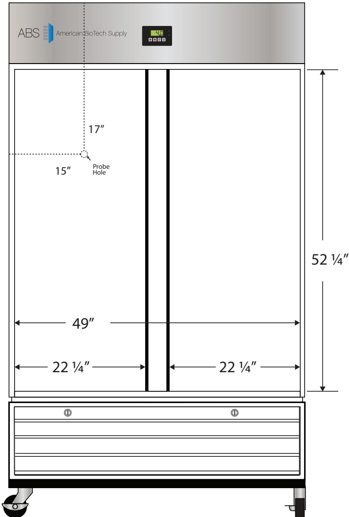
Front View
