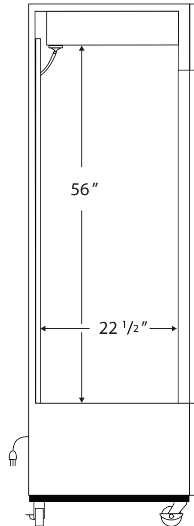
Side View
