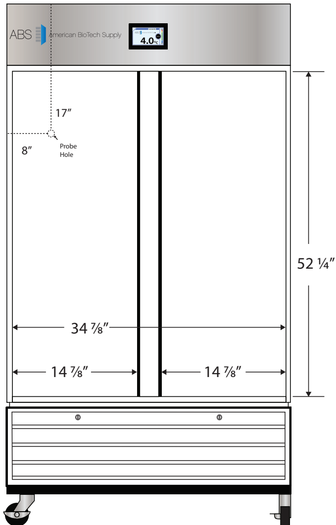
Front View
