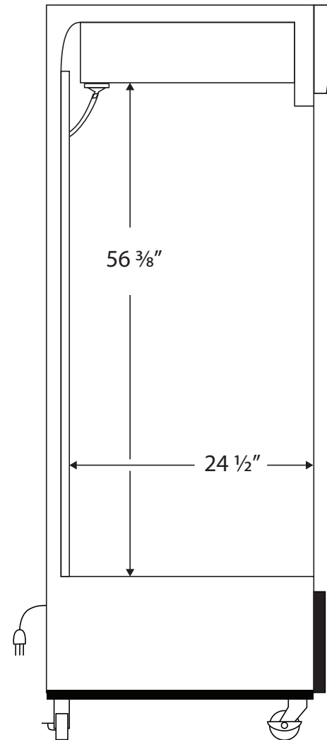
Side View
